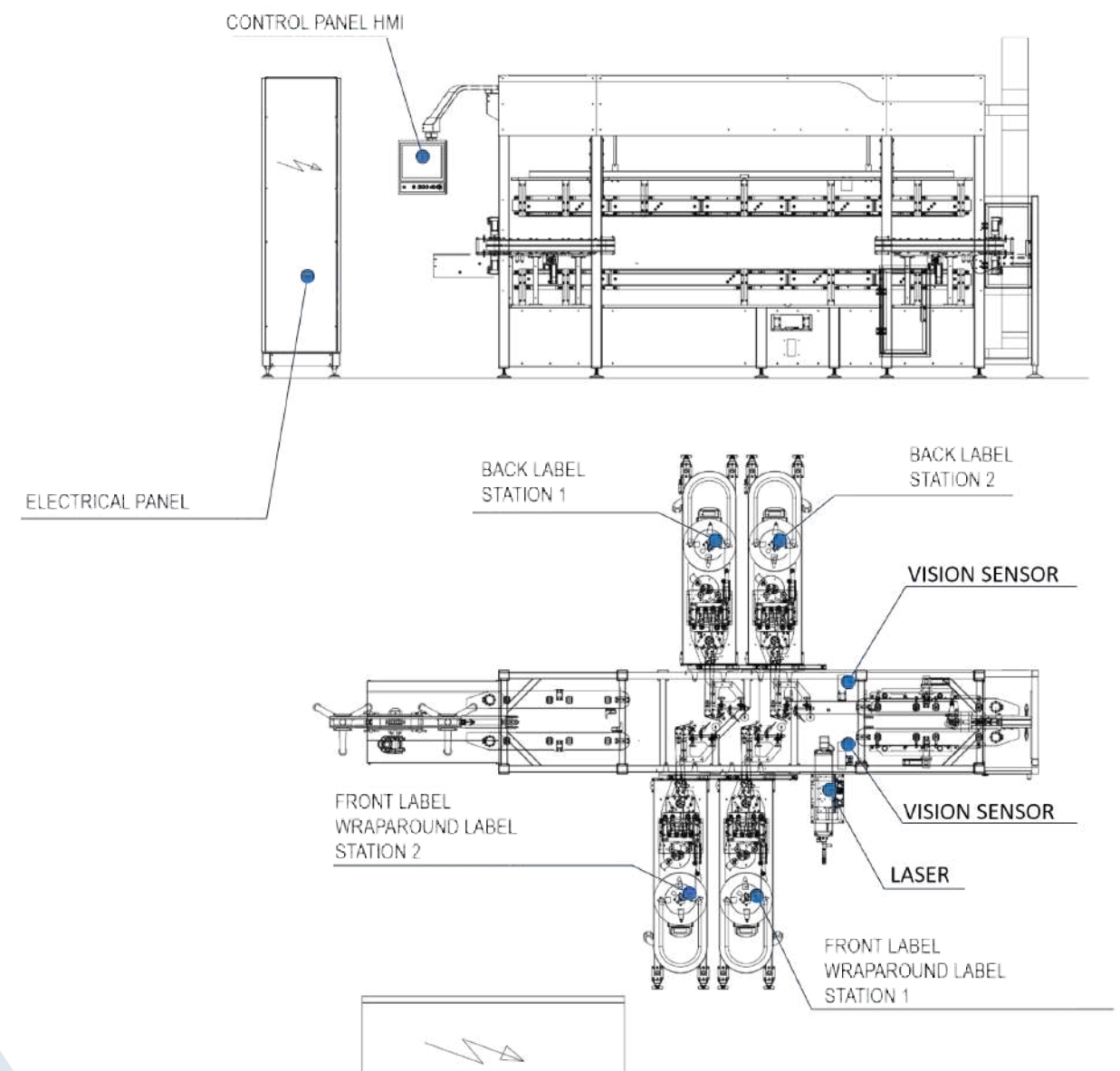
Example layout with machine configuration with 4 stations
